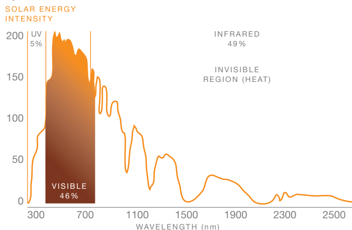
FIG. 1 - SPECTRUM OF SOLAR RADIANCE.
