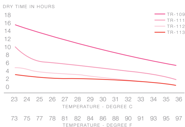
Eclipse® dry time vs. temperature at 50% relative humidity
